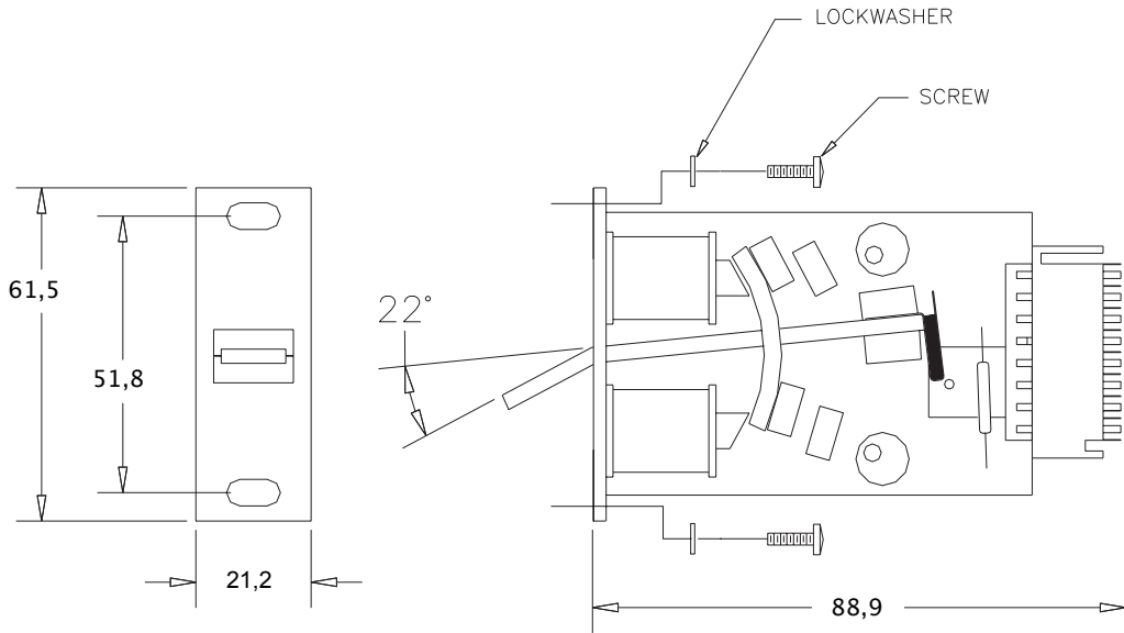
Power Tab Dimensions (mm)
